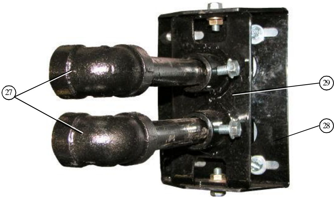
26" & 28" Vaporizer coil connection and adjustment brackets.
